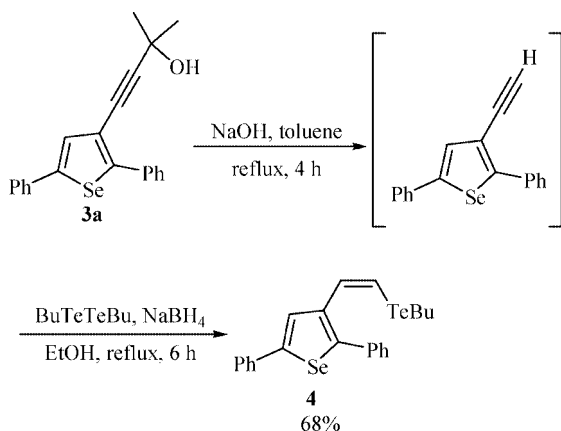
Scheme 2. Synthesis of vinylic telluride 4 .
